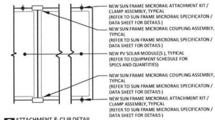
ATTACHMENT & CLIP DETAIL SCALE: NOT TO SCALE
