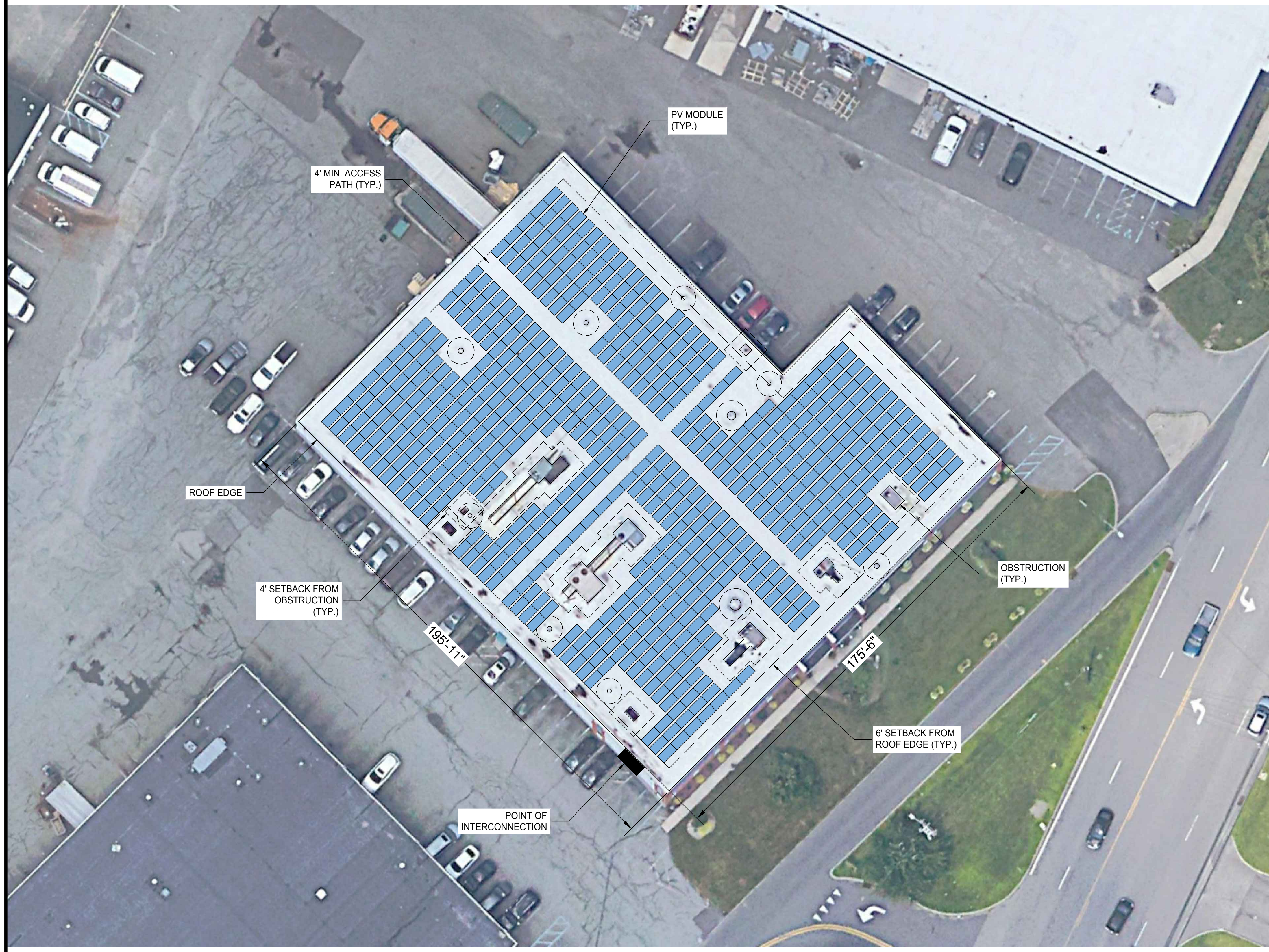
1 G-100 GENERAL SITE PLAN 1" = 20'
